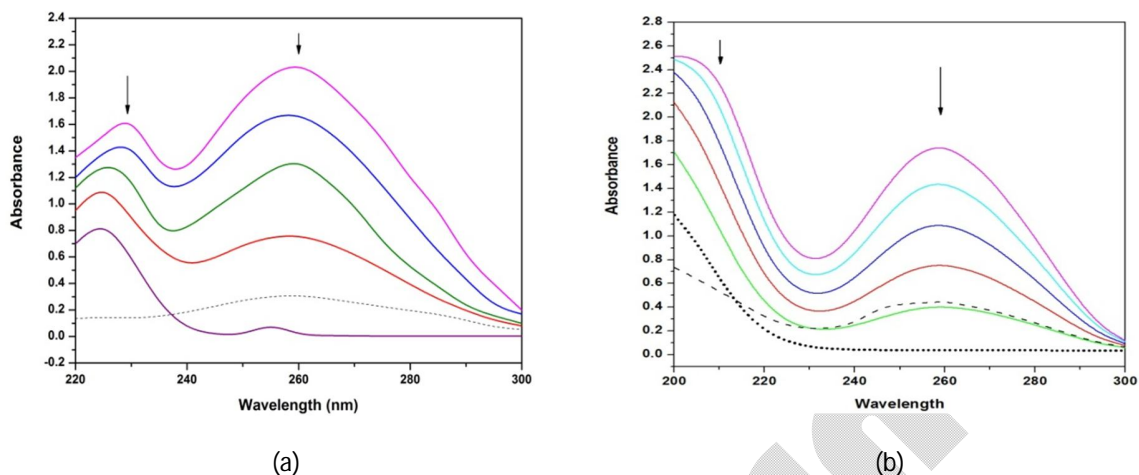
Figure 3. Absorption spectra of (a) complex 1 and (b) complex 3 , in Tris-HCl buffer upon addition of DNA = 0.5 \mu\text{M} , 0-100 \mu\text{l} . Arrow shows the absorbance change upon increasing the concentration of DNA.
