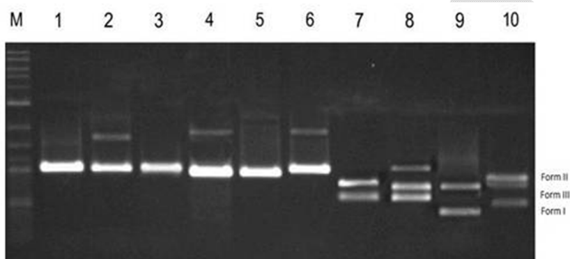
Figure 5. Cleavage of supercoiled pUC19 DNA (0.5 \mu g) by the ligands and complexes 2 and 4 in a buffer containing 50 mM Tris-HCl at 37 ^{\circ} C (30 min): lane M: marker; lane 1: DNA control; lane 2: DNA + H_2O_2 ; lane 3: L^1 ( 10^{-3} M) + DNA; lane 4: L^1 + DNA + H_2O_2 ; lane 5: L^2 + DNA; lane 6: L^2 + DNA + H_2O_2 ; lane 7: complex 2 ( 10^{-3} M) + DNA; lane 8: complex 2 + DNA + H_2O_2 ; lane 9: complex 4 + DNA; lane 10: complex 4 + DNA + H_2O_2 .
