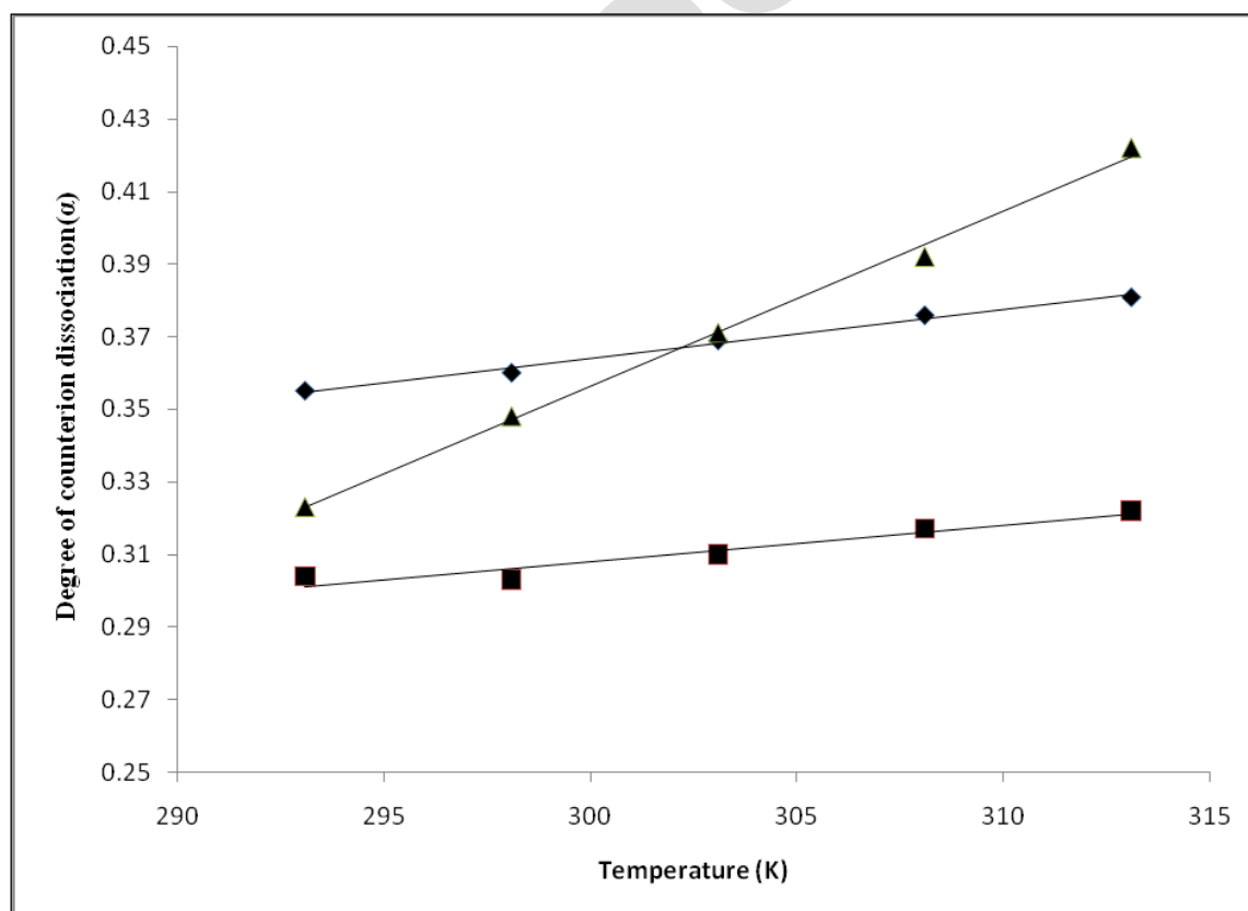
Figure 3: The plot of degree of counterions of dissociation ( \alpha ) against temperature in 0.17 mass fraction ( \omega_s ) of organic solvent ( \diamond = EG + Water, \blacksquare = DMSO + Water, \blacktriangle = DMF + Water).
