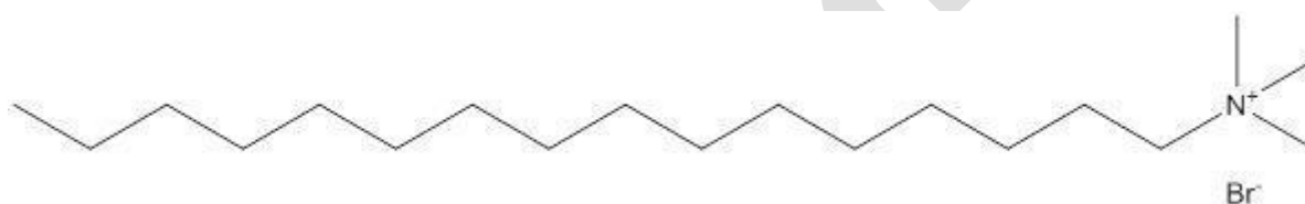
Figure 1: Schematic representation of CTABr molecular structure.
