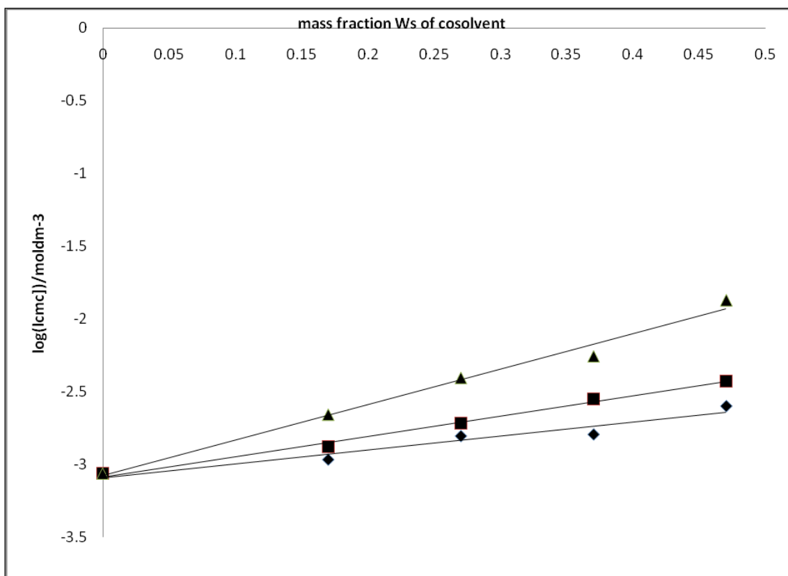
Figure 2: Plot of \log([\text{cmc}]/\text{mol dm}^{-3}) against the mass fraction ( \omega_s ) of the organic solvent at 293.1 K ( \blacklozenge = EG + Water, \blacksquare = DMSO + Water, \blacktriangle = DMF + Water).
