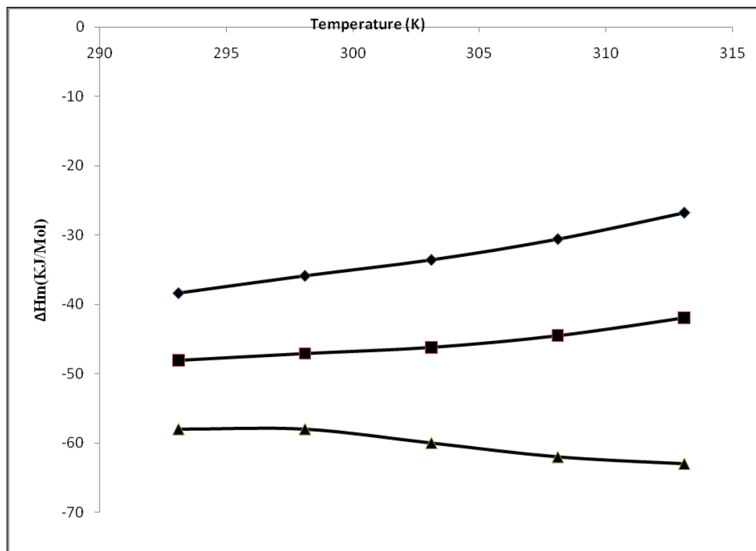
Figure 4: The change in enthalpy ( \Delta H_m^\circ KJ mol -1 ) against temperature in 0.17 mass fraction ( \omega_s ) of organic solvent ( \blacklozenge = EG + Water, \blacksquare = DMSO + Water; \blacktriangle = DMF + Water).
