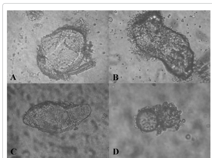
Figure 1: Ascocotyle longa metacercariae inactivated by heating observed in microscopy. 100X. A, B, and C: different larvae forms, D: cysts.
