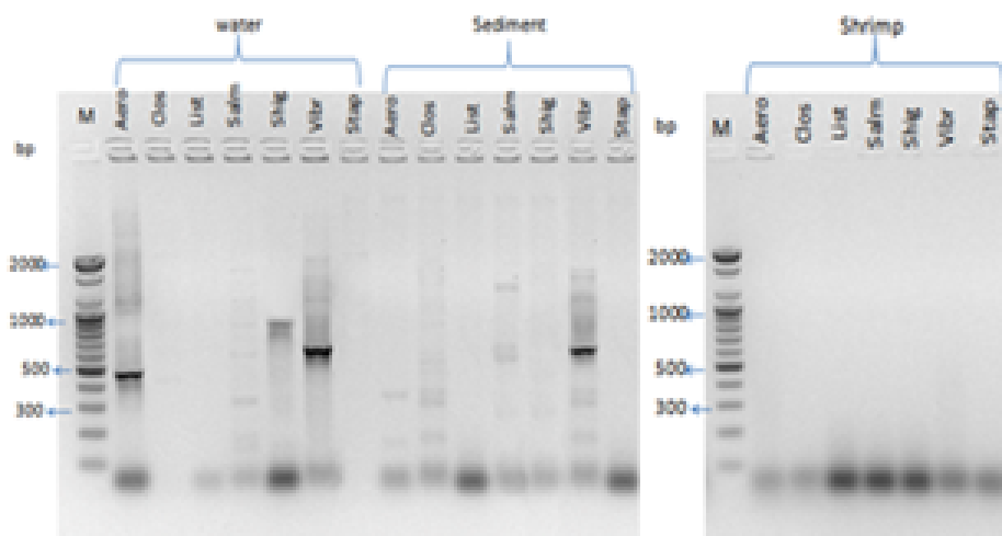
Figure 6: UV visualization of PCR product of farm 5 following electrophoresis in a 2% agarose gel. Lanes 1 to 7 and 8 to 14 represent water, sediment respectively where 7 primers (Aero, Clos, List, Salm, Shig, Vibr, Stap) is used for each sample. For intestine of shrimp sample Lane 1 to 7 which represent Aero , Clos , List , Salm , Shig , Vibr , Stap serially. Lane M represents 100 bp DNA ladder or marker.
