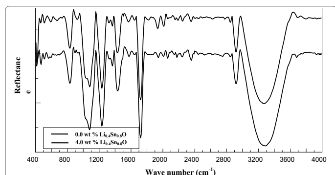
Figure 1: FTIR reflectance spectra of PVA nanocomposite films with (a) 0, (b) 0.5, (c) 1.0, (d) 2.0, and (e) 4.0 wt % of \text{Li}_{0.4}\text{Sn}_{0.8}\text{O} .
