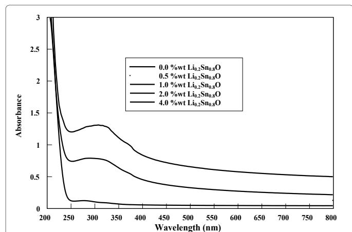
Figure 2: UV-visible absorbance spectra of PVA nanocomposites with (a) 0, (b) 0.5, (c) 1.0, (d) 2.0, and (e) 4.0 wt % of \text{Li}_{0.4}\text{Sn}_{0.8}\text{O} .
