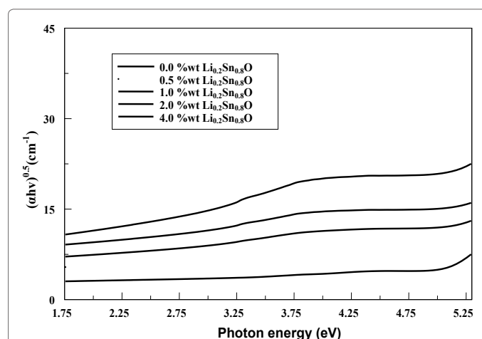
Figure 4: Tauc's plot for the determination of direct band gaps.
