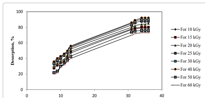
Figure 12: Effect of 0.4% citric acid on desorption of water of PVA hydrogel at various radiation doses.
